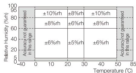
HUMIDITY SENSOR Z2000
