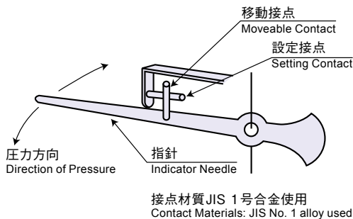
Electric Pointer Contact Switch Structure
